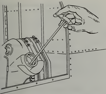
FIGURE 6-17. Checking oil level with dipstick.
